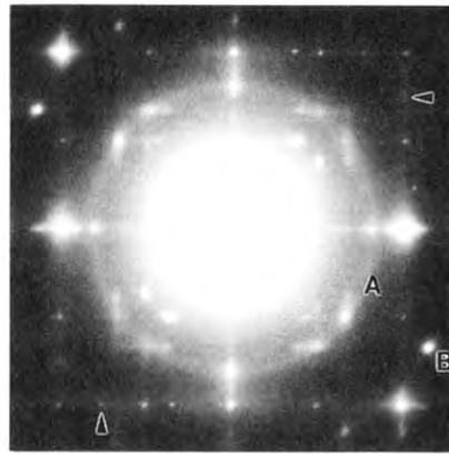
FIG. 1. A typical TED pattern following Ag deposition on a Si(100)-(2 \times 1) surface; arrowed surface reconstruction spots coexist with the (111) and (220) rings of Ag, denoted by the letters A and B . All features can be interpreted by a combination of silicon, silver, and moiré spacings.
