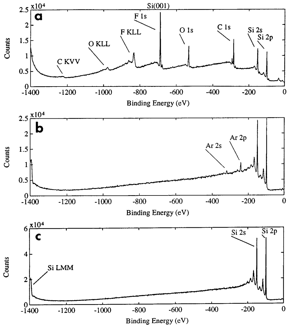
FIG. 1. XPS spectrum of an (a) as-etched Si(001) surface, (b) after argon milling, and (c) after annealing.
