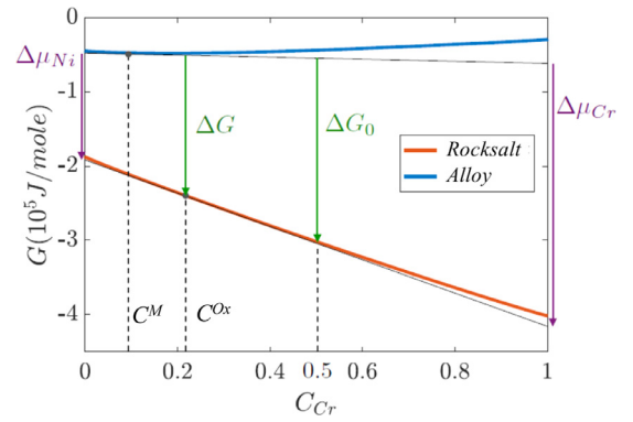
Fig. 3. Free energy versus composition curves for the alloy and rocksalt oxide at T=1000\text{ K} and atmospheric oxygen effective pressure. The free energy is plotted in units of joules per mole of nickel and chromium. The oxygen in the oxide is in equilibrium with the atmosphere. The driving force for oxidation, \Delta G , for alloy composition C^M and oxide composition C^{\text{Ox}} is constructed graphically. It is given by the vertical distance between the tangent line of the alloy free energy curve at C^M and the free energy curve of the rocksalt oxide. A characteristic driving force \Delta G_0 for the formation of oxide of composition C_{\text{Cr}}=0.5 from a metal of composition C_{\text{Cr}}=0.1 also shown. The chemical potential of each component decreases upon the formation of the oxide, as shows by the arrows at C_{\text{Cr}}=0.1 .
