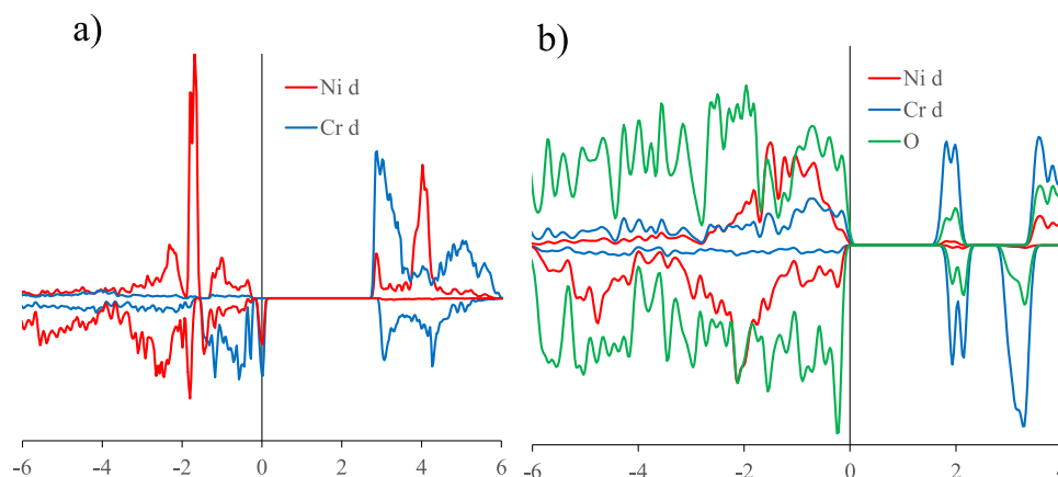
Fig. 9. Density of states for corundum structures with \text{Ni}^{3+} : in (a) \text{NiCr}_{15}\text{O}_{24} and (b) \text{NiCrO}_3 , color coded according to the legend; both are discussed further in the text. Up spins are above the axis and down spins below, with the x axis is in eV using the Fermi energy as the origin, y-axis is unitless. (For interpretation of the references to color in this figure legend, the reader is referred to the web version of this article.)
