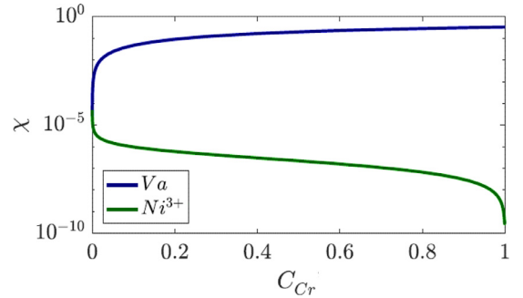
Fig. 4. Vacancy and \text{Ni}^{3+} concentration in the rocksalt oxide as a function of chromium content at T=1000\text{ K} and atmospheric effective oxygen pressure. The concentration curves satisfy valence neutrality and oxygen equilibrium with the gas phase.
