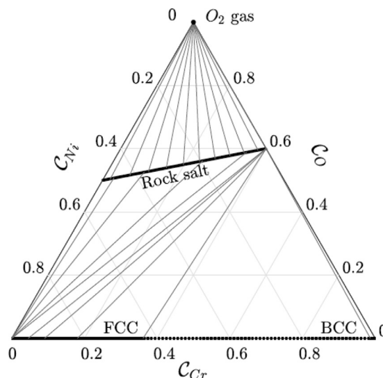
Fig. 2. Ternary phase diagram of the Ni–Cr–O system at T = 1000 K and atmospheric pO_2 with the corundum and spinel oxide phases removed, calculated from [44]. The light grey lines are tie lines in the two-phase regions. The dotted line on the C_{Cr} axis is the two-phase region in the pure alloy.
